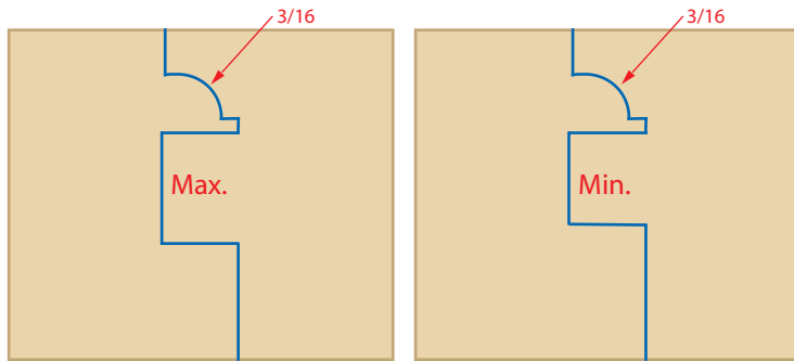
1/2" plywood
