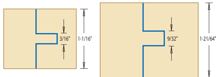
SC555 INSTILE & RAIL SYSTEM
