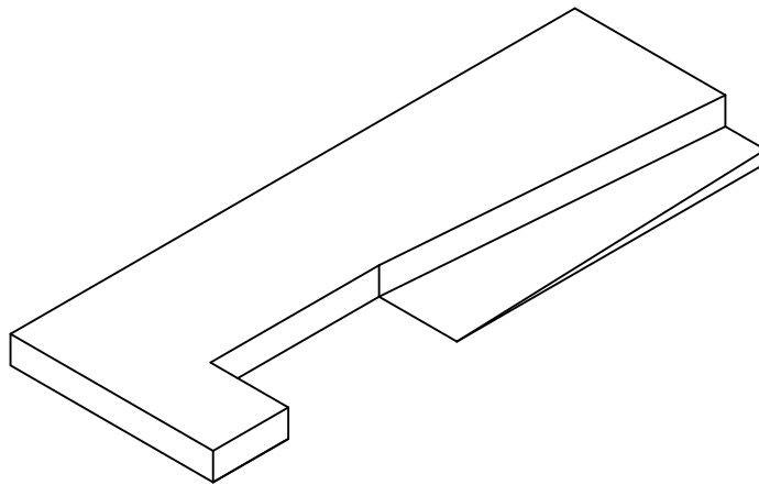
Jig for shaping octagonal tapers with a table-mounted router
