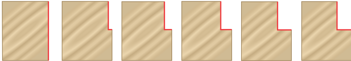
Flush rabbet use #67398 collar
